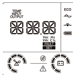
Figura 2 -4 Panel LCD
